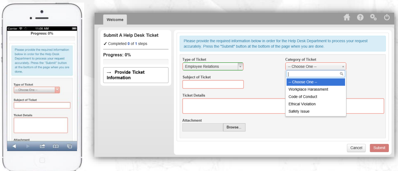
Figure 2. Screenshot of the unified UNiTY UE (User Experience) representing a Case/Ticket Management Process.
